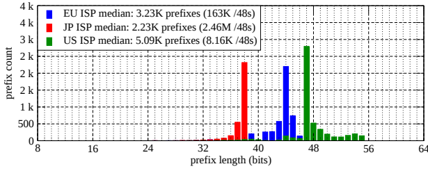
Figure 1: Anonymous aggregate histogram: k = 256
